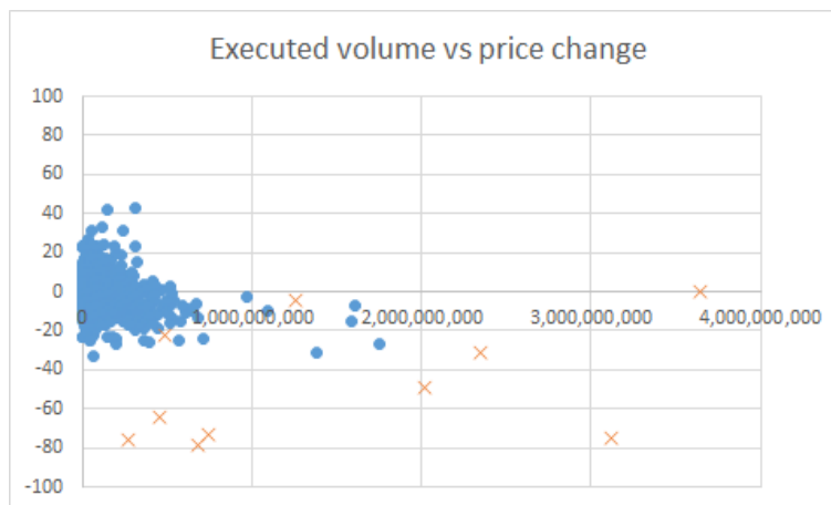
Figure 7: Executed volumes vs price changes, 8th July
