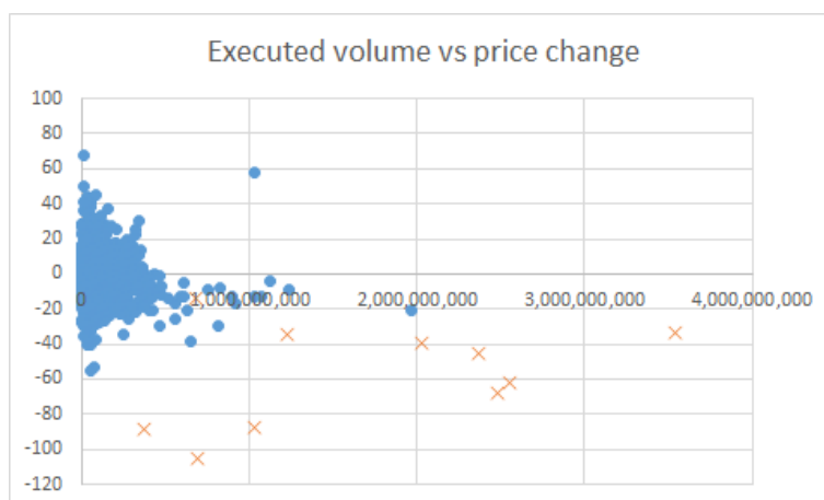
Figure 5: Executed volumes vs price changes, 24th August
