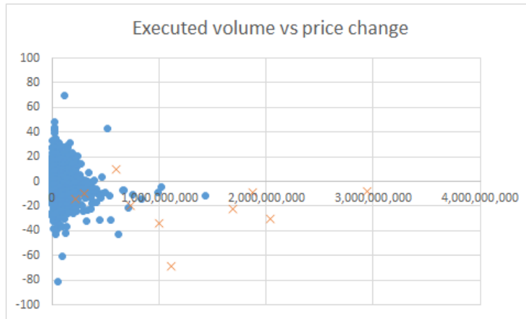
Figure 2: Executed volumes vs price changes, 4th September
