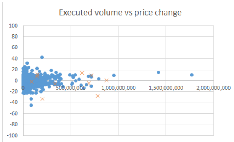
Figure 9: Executed volumes vs price changes, 17th July
