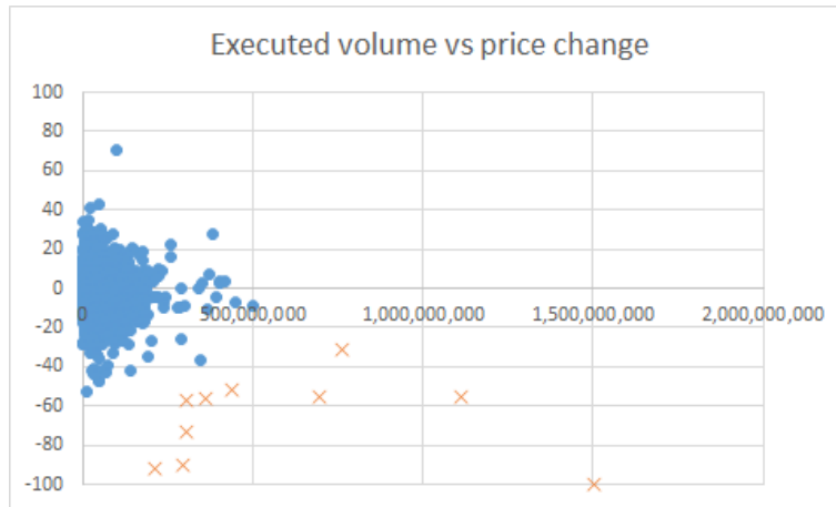
Figure 3: Executed volumes vs price changes, 8th September
