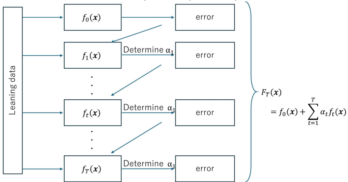
Figure 30: Image of boosting
